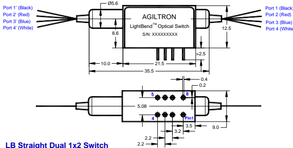
LB Straight Dual 1x2 Switch
